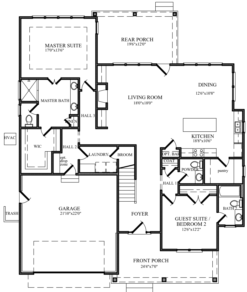
1,875 sq. ft. · First Floor
