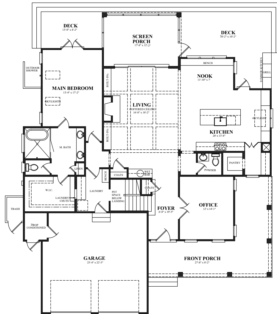
FIRST FLOOR PLAN - 1899 s.f.
