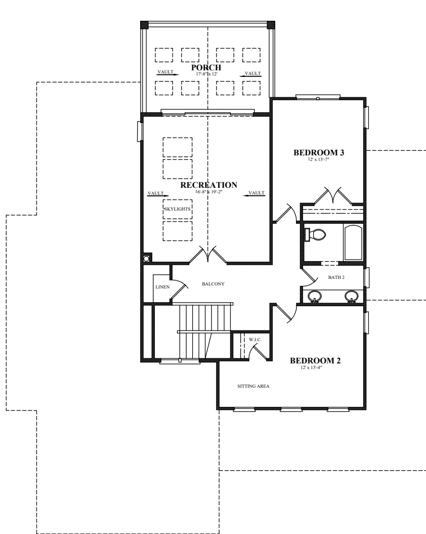
SECOND FLOOR PLAN - 1052 s.f.
