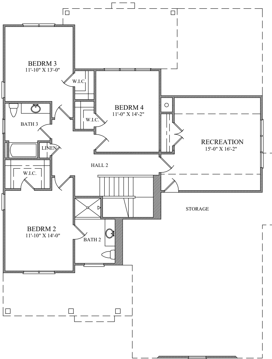
1,225 sq. ft. Second Floor
