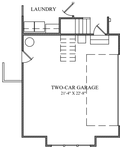
Optional Bonus First Floor . 2,465 sq. ft.
