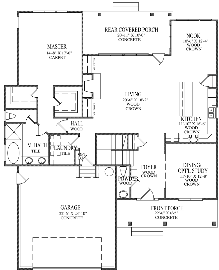
First Floor . 1,707 sq. ft.
