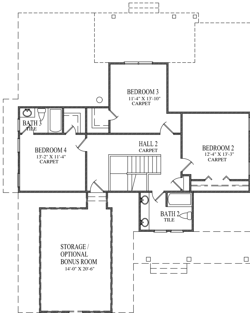
Second Floor . 920 sq. ft.
