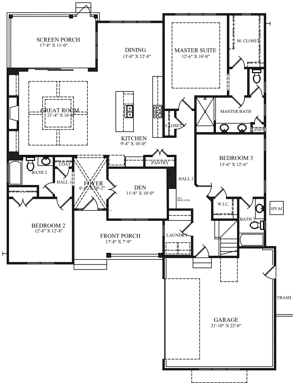
2,153 sq. ft. · First Floor
