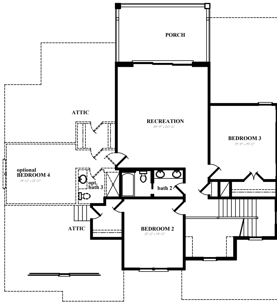
SECOND FLOOR PLAN - 1043 s.f. OPT. BEDROOM 4 / BATH 3 - 318 s.f.
