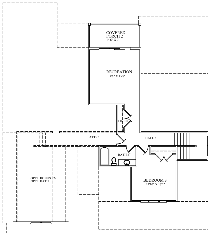
648 sq. ft. • Second Floor
